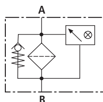
Pressure filter
